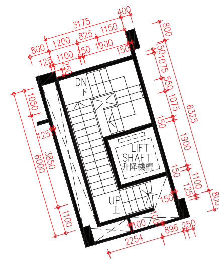
Part Plan of Upper Part of Lower Ground Floor 低層地下上方之部分平面圖
